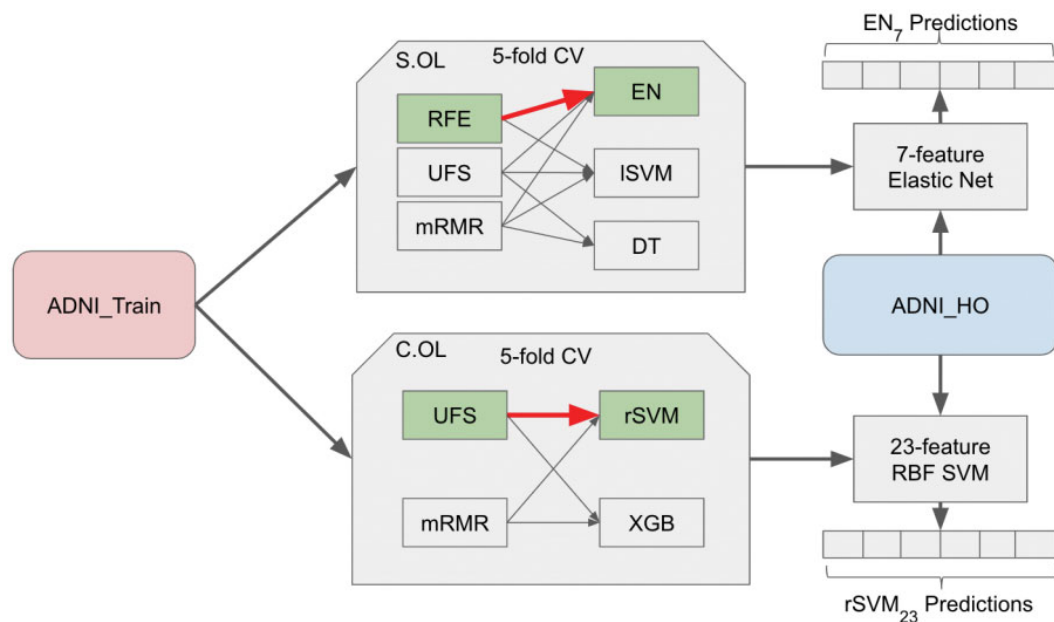
Figure 1. Our overall framework: Left-to-right is the training component, to produce both a simple classifier (here EN_7 , on top, using S.OL) and a complicated classifier (here rSVM_{23} , on bottom, using C.OL). Each of these OLs considered a set of feature selection methods, from \{RFE, UFS, mRMR\} , and a given set of possible base-learners – S.OL considered EN, lSVM and DT, while C.OL: rSVM and XGB. (Note that DT did not use RFE). The RED arrow, in each, is the combination of feature selection method and base-learner with the best 5-fold cross-validation accuracy. We then evaluated each of these classifiers, by running each on the (data from) ADNI_HO (vertical, on right)
