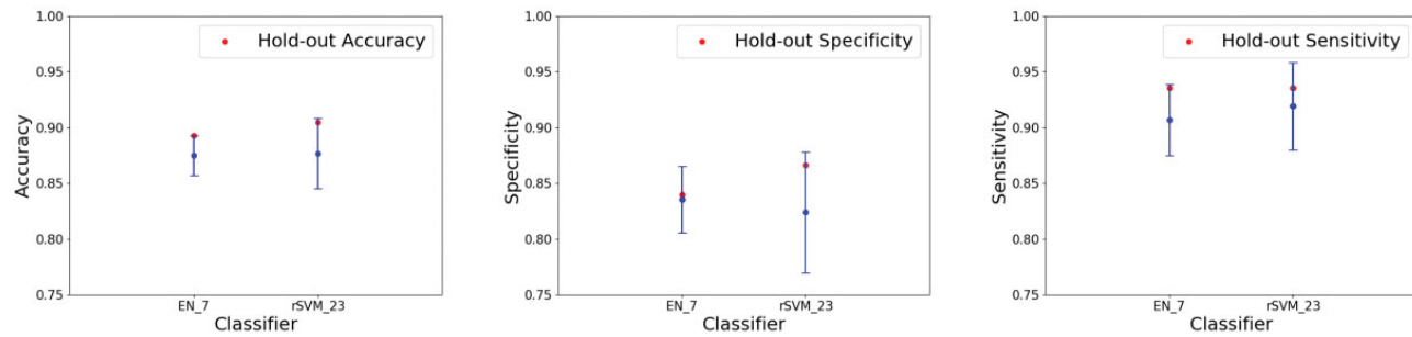
Figure 2. Mean and standard deviation (STD) of the 5-fold cross-validation (CV) performance of EN 7 and rSVM 23 models, on ADNI_TRAIN. The red dots show the hold-out performance of these models, on ADNI_HO.
