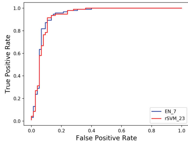
Figure 3. The receiver operation curve (ROC) for our EN 7 and rSVM 23 models
